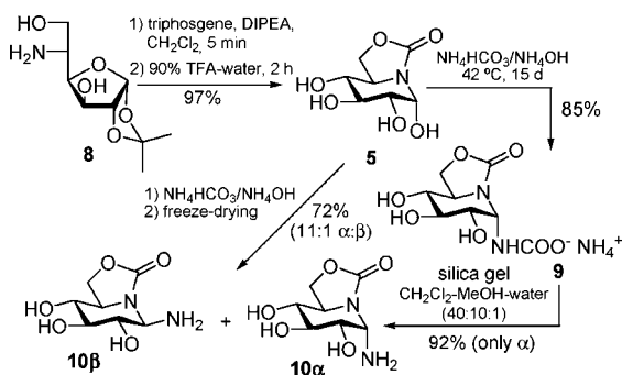
Scheme 1. Synthesis of Configurationally Stable \alpha -D-Glucopyranosylamine Mimics with gem -Diamine Structure
