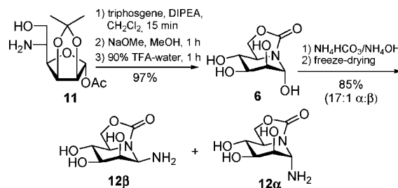
Scheme 2. Synthesis of Configurationally Stable \alpha -D-Mannopyranosylamine Mimics with gem -Diamine Structure
