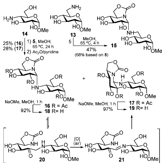
Scheme 3. Synthesis of \alpha - N -Linked Disaccharide Mimics
