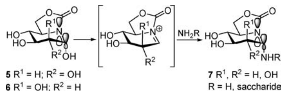
Figure 2. Structures of sp^2 -iminosugars with hemiaminal ( 5 , 6 ) and gem -diamine-type pseudoanomeric centers ( 7 ). The orbitals involved in the negative hyperconjugation contribution to the GAE and the presumably structure of the azacarbonium ion intermediate are shown.
