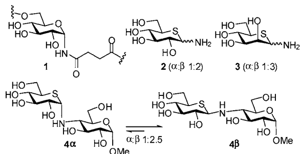
Figure 1. Partial structure of the \alpha - N -glycopeptide nephritogenoside ( 1 ) and structures of 5-thiogluco(manno)pyranosylamines ( 2 and 3 ) and of the N -linked pseudodisaccharide 4 , with indication of the anomeric ratio.
